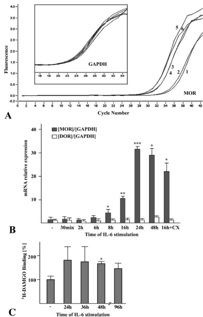
Fig. 1. Effect of interleukin-6 (IL-6) on μ- and δ-opioid receptor expression in SH SY5Y cells. A and B, effects on mRNA. SH SY5Y cells were stimulated with interleukin-6 (9 ng/ml) for different periods of time and then subjected to real-time RT-PCR. A, one representative experiment of a real-time RT-PCR monitoring amplification of μ-opioid receptor transcripts (1 and 2, unstimulated controls; 3 and 4, 16-h interleukin-6; 5 and 6, 16-h interleukin-6 and cycloheximide). Inset, amplification of GAPDH mRNA of the same cDNAs is plotted. B, quantification of the results normalized to GAPDH. Results are expressed as fold induction (■, [μ-opioid receptor(MOR)]/[GAPDH]; □, [δ-opioid receptor(DOR)]/[GAPDH]). The 16-h incubations were tested with and without cycloheximide (CX). The results of three independent experiments performed in triplicate plus S.E.M. are shown. *, p < 0.05; **, p < 0.01; ***, p < 0.001. C, relative [ 3 H]DAMGO binding after incubation of cells for different periods of time with interleukin-6 (9 ng/ml). For the controls, 100% equals to an average of 52 fmol of binding sites per milligram of protein. The results of two independent experiments performed in triplicate plus S.E.M. are shown. *, p < 0.05.
